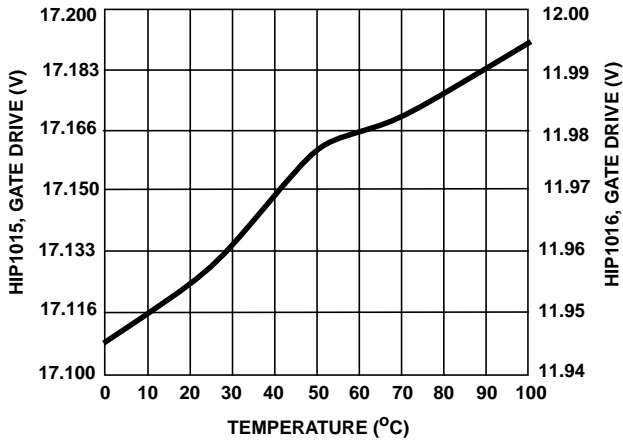
FIGURE 9. GATE DRIVE VOLTAGE, VDD = 12V
