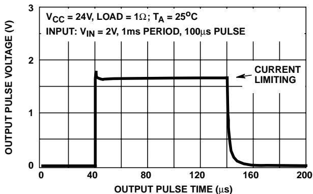
FIGURE 7. TYPICAL OUTPUT CURRENT PULSE WHEN SWITCHING INTO A LOW IMPEDANCE ( 1\Omega ), OR SHORTED LOAD. FOR THE CONDITIONS SHOWN, OUTPUT CURRENT LIMITING IS \sim 1.7A
