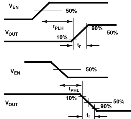
SWITCHING WAVEFORMS
