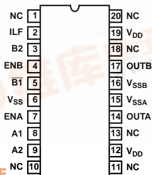
HIP4020 SOIC TOP VIEW
