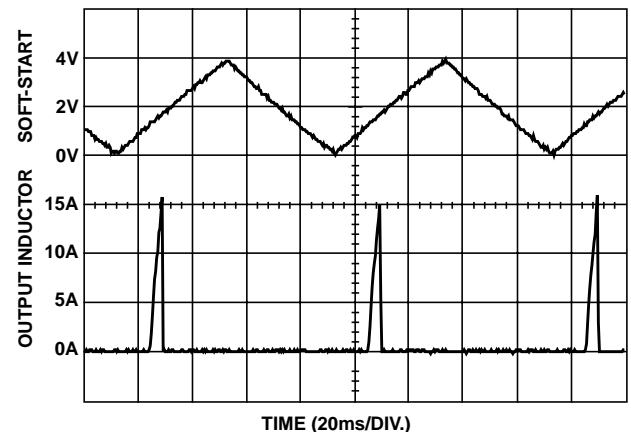
FIGURE 4. OVER-CURRENT OPERATION
