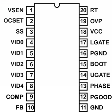
HIP6004 (SOIC) TOP VIEW
