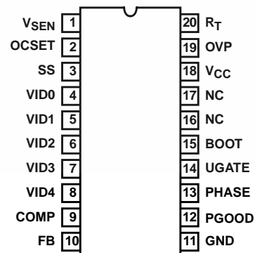
HIP6005A (SOIC) TOP VIEW
