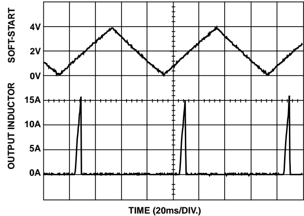
FIGURE 4. OVER-CURRENT OPERATION
