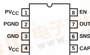
HIP6201 (SOIC) TOP VIEW
