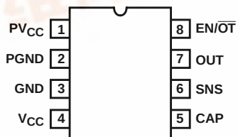
HIP6200 (SOIC) TOP VIEW
