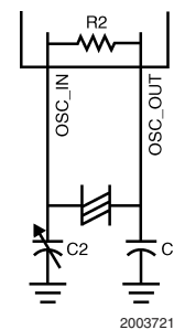
FIGURE 2. Crystal Oscillator
