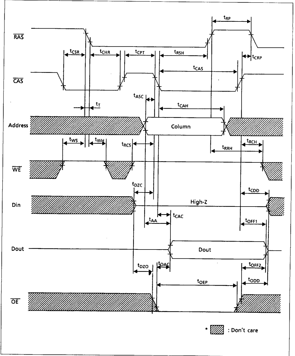
CAS-Before-RAS Refresh Counter Check Cycle (Read)
