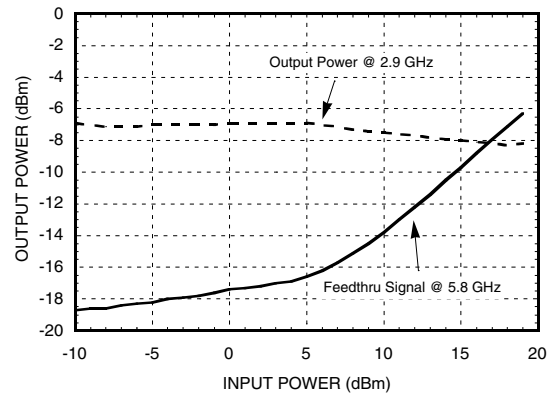
Output Power vs. Input Power, Input Frequency= 5.8 GHz
