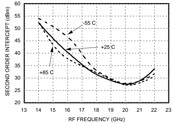
Input IP2 vs. Temperature @ LO = 0 dBm
