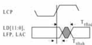
TFT Mode Signal Delay
