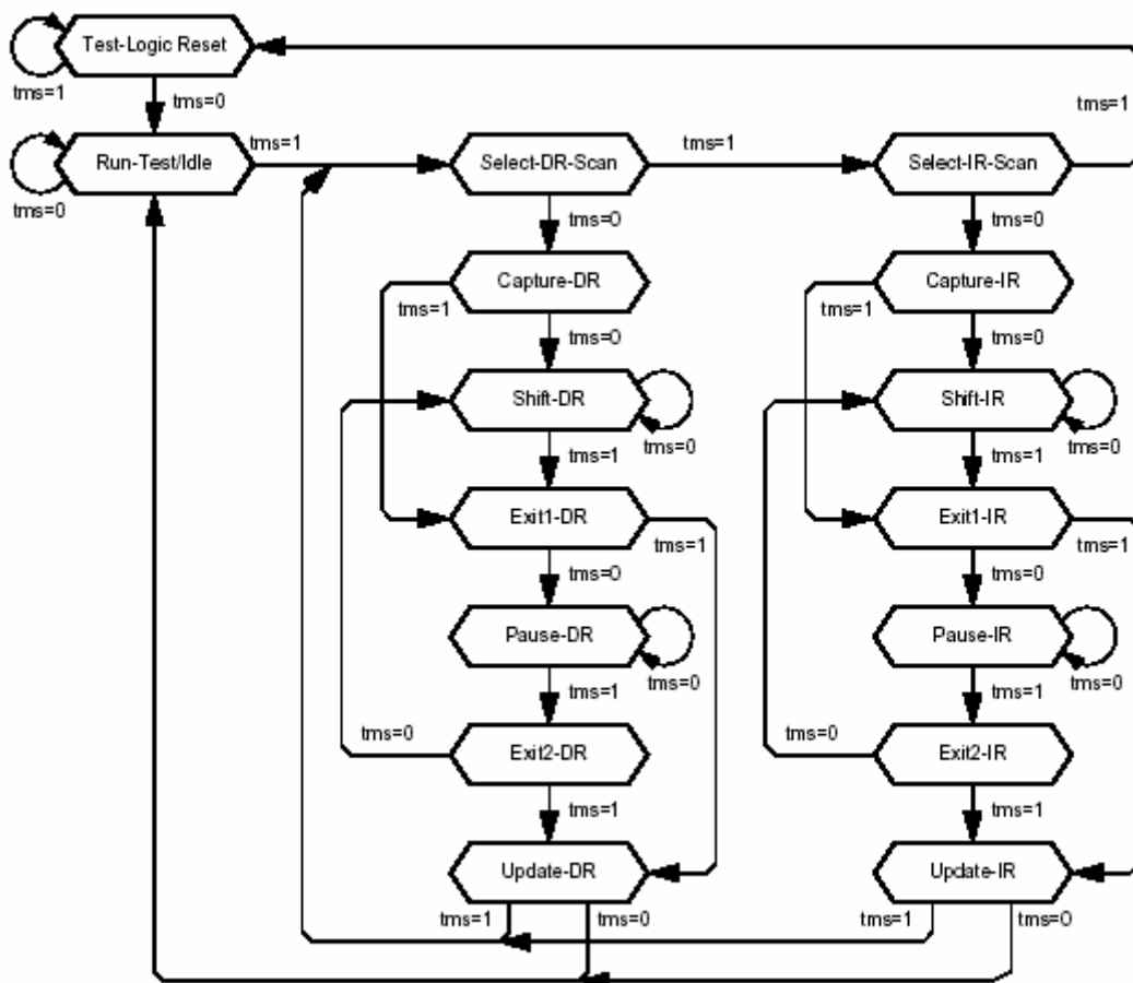
Figure 11-1: Test Access Port (TAP) Controller State Transitions
