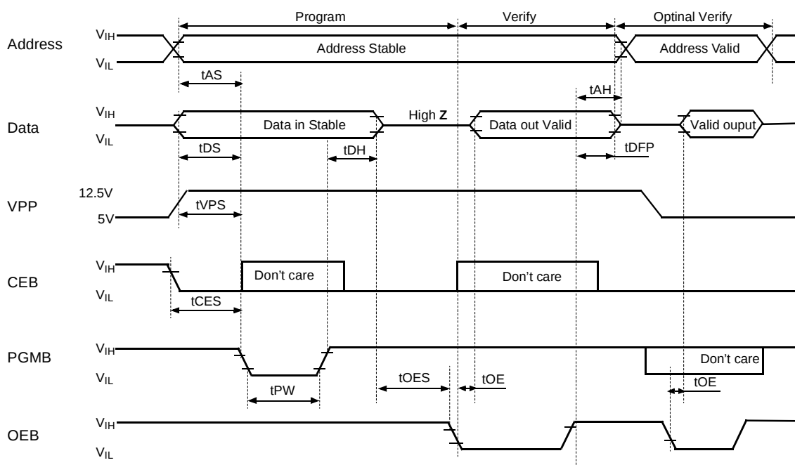
Figure 23-7 Figure Programming Timing Chart
