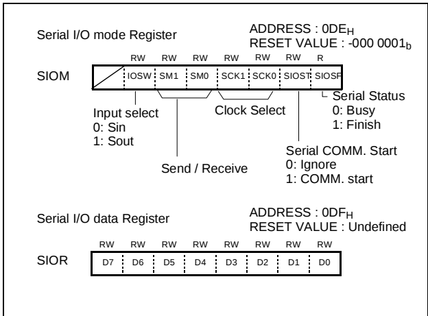
Figure 13-2 Serial I/O Registers
