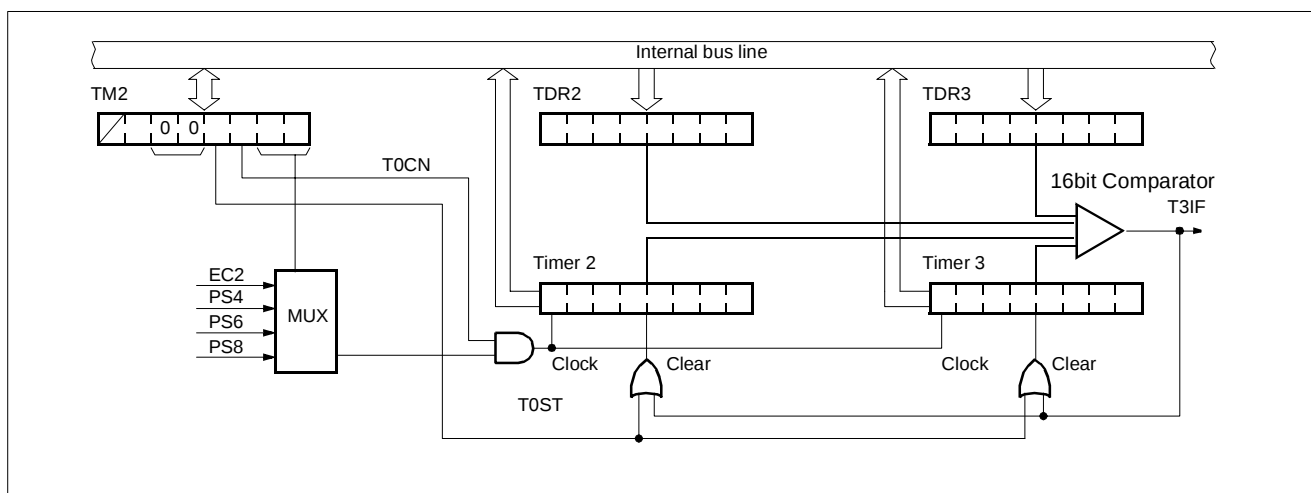
Figure 11-8 Simplified Block Diagram of 16bit Timer/Event Counter 2,3
