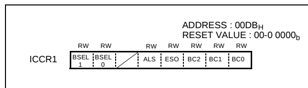
Figure 18-5 I 2 C control Register 1
