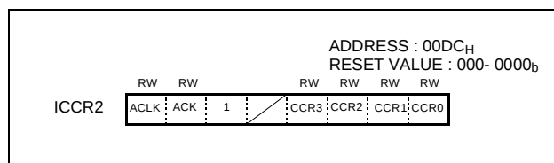
Figure 18-6 I²C control Register 2
