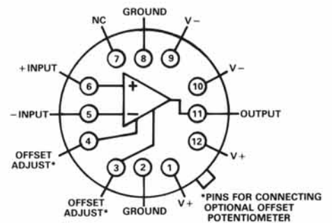
TO-8 PACKAGE BOTTOM VIEW
