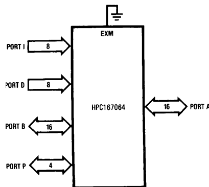
FIGURE 15. Single-Chip Mode
