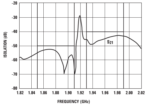
Figure 8. S21, Isolation (typical).
