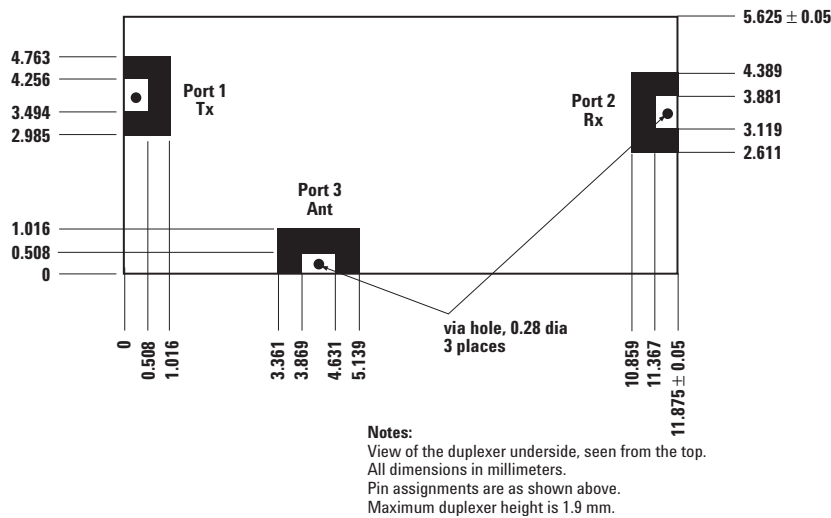
Figure 12. Outline Drawing.
