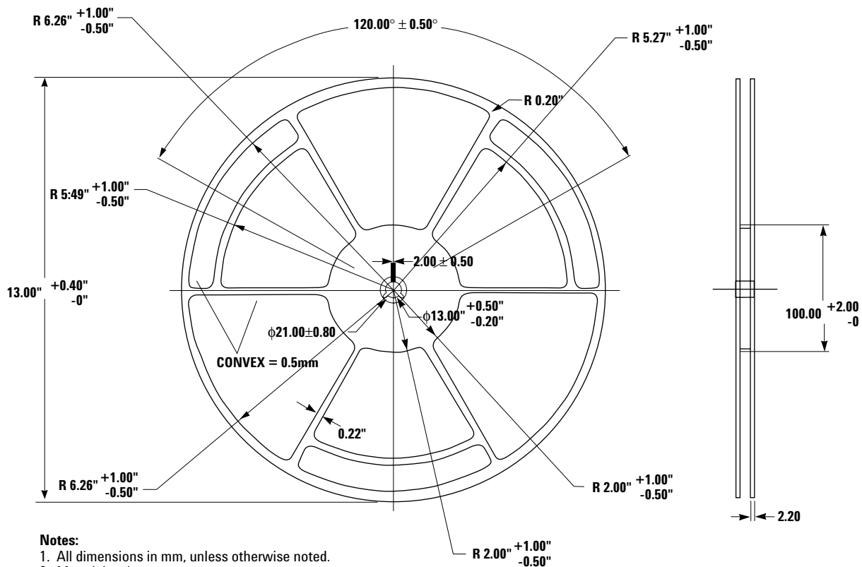
Figure 14. Reel Drawing.
