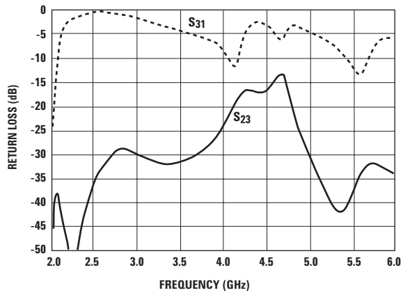
Figure 9. Wideband Insertion Loss (typical).
