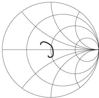
Figure 5. S_{11} , Tx Port Impedance (typical).
