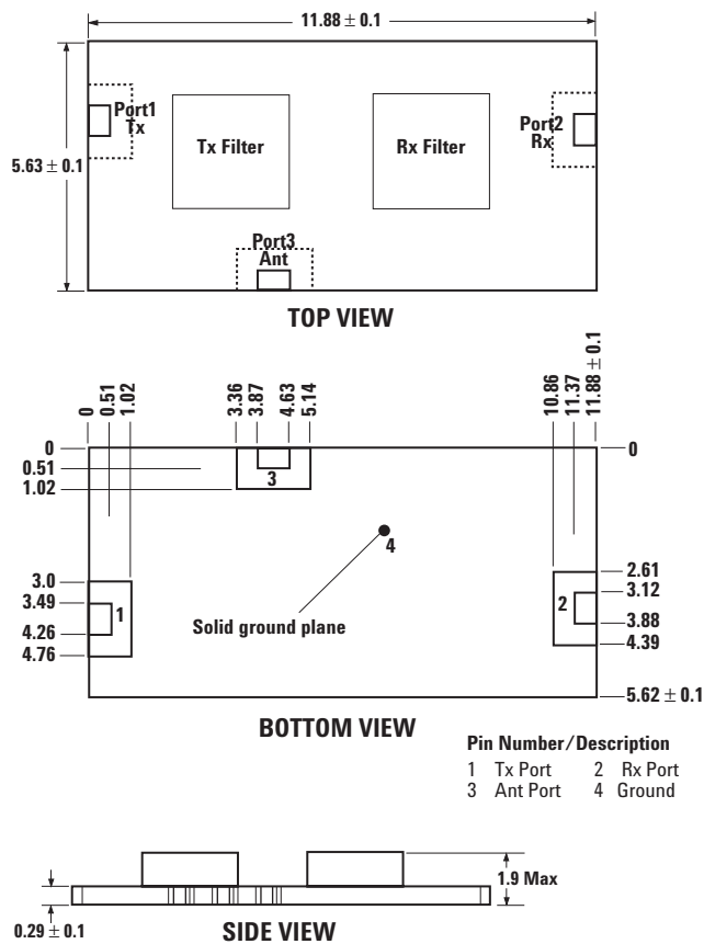
Figure 12. Outline Drawing.
