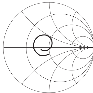
Figure 6. S_{22} , Rx Port Impedance (typical).
