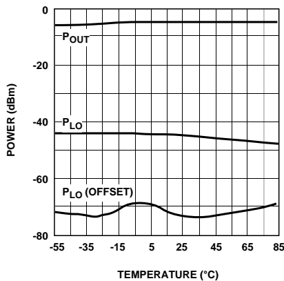
Figure 29. LO Leakage with No DC Offsets at 100\text{ MHz} vs. Temperature (Upper Curve) and LO Leakage with DC Offsets Adjusted for Minimum Leakage at 25^\circ\text{C} vs. Temperature (Lower Curve). V_{CC} = 5\text{ V} , LO = -12\text{ dBm} , V_{Iref} = V_{Qref} = 2.5\text{ V} .
