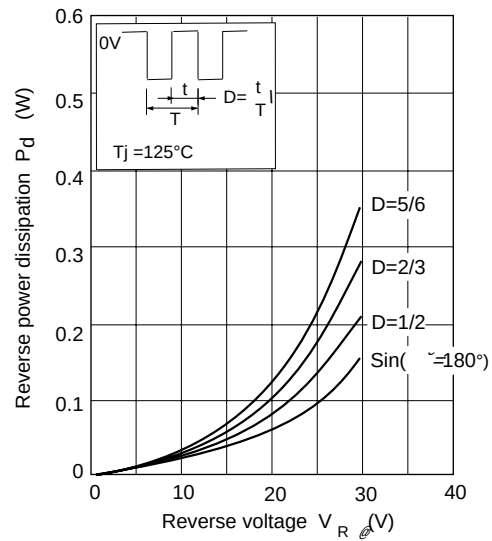
Fig.4 Reverse power dissipation Vs. Reverse voltage
