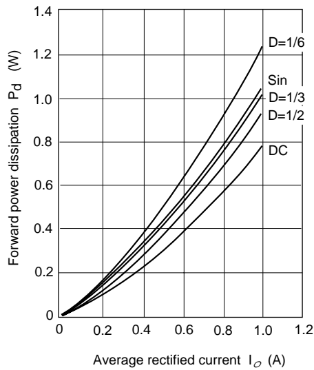
Fig.1 Forward power dissipation Vs. Average rectified current
