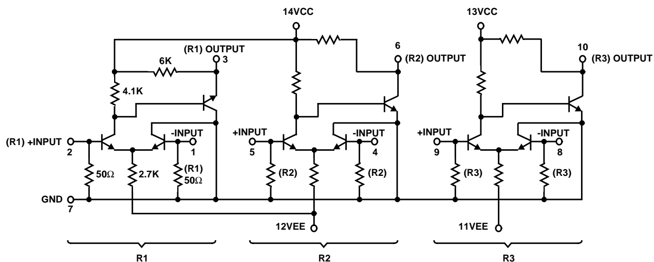
FIGURE 7. HS-246RH, HS-248RH
