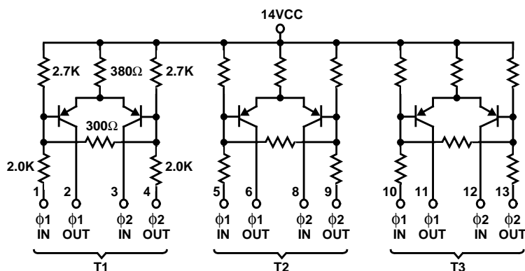
FIGURE 6. HS-245RH
