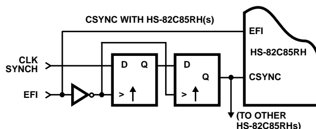
FIGURE 23. CSYNC SYNCHRONIZATION METHODS
