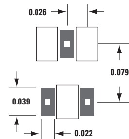
Figure 6. Recommended PCB Pad Layout for Agilent's SC70 3L/SOT-323 Products.
