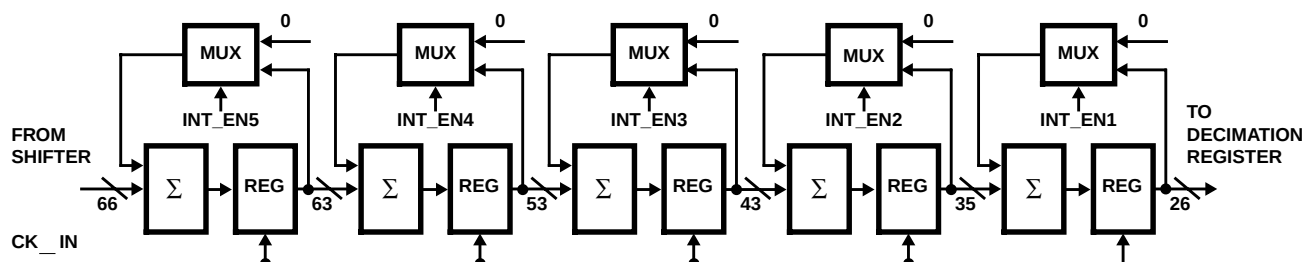
FIGURE 2. INTEGRATOR
