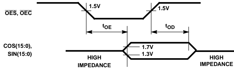
FIGURE 12. OUTPUT ENABLE, DISABLE TIMING
