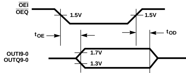
FIGURE 29. OUTPUT ENABLE/DISABLE
