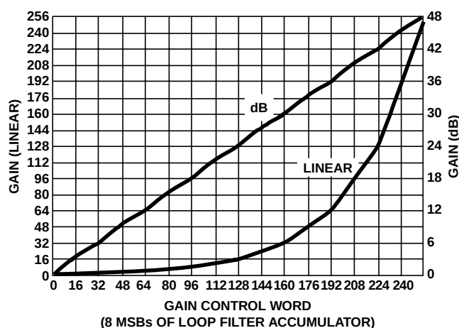
FIGURE 5. GAIN CONTROL TRANSFER FUNCTION
