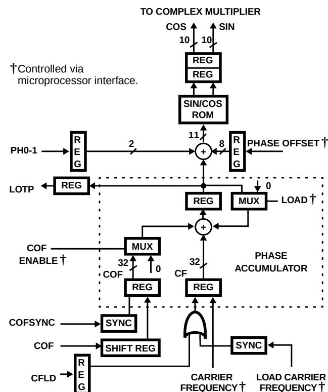
FIGURE 2. SYNTHESIZER NCO
