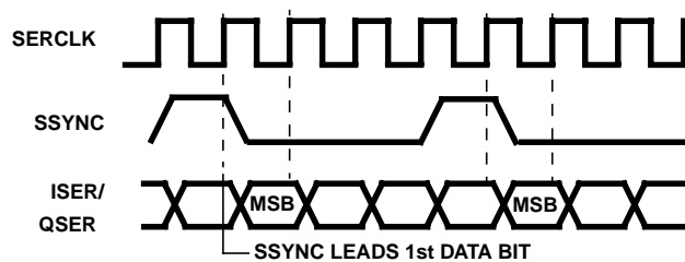
FIGURE 2. SERIAL INPUT TIMING FOR ISER AND QSER INPUTS
