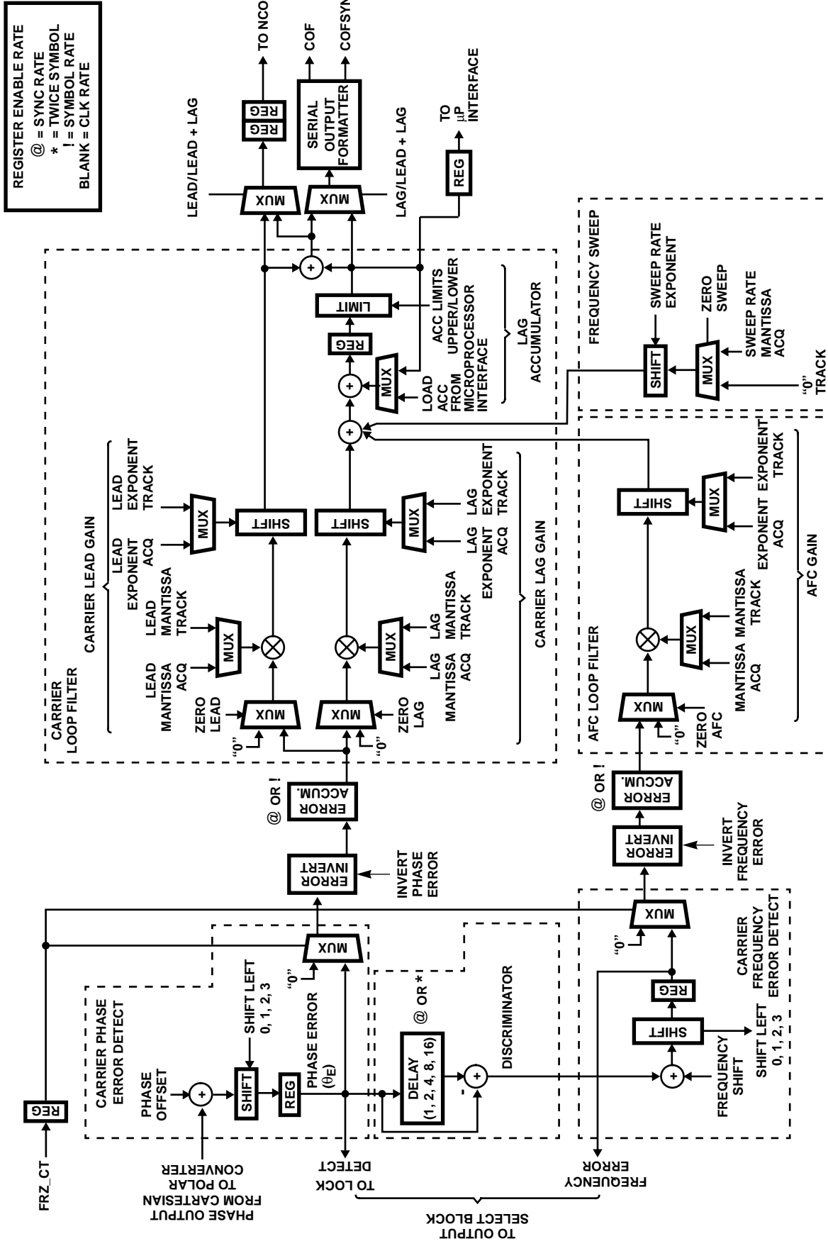
FIGURE 15. CARRIER ACQUISITION/TRACKING LOOP BLOCK DIAGRAM
