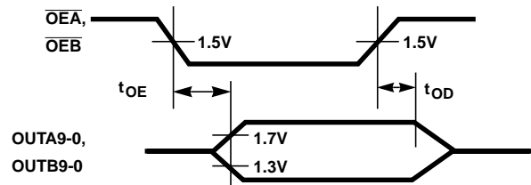
FIGURE 29. OUTPUT ENABLE/DISABLE
