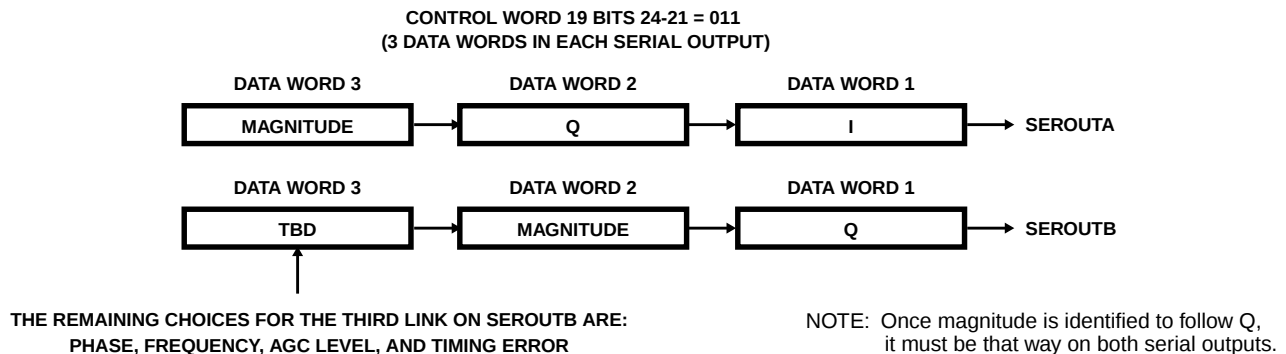
FIGURE 32. EXAMPLE 2 SERIAL OUTPUT DATA STREAM
