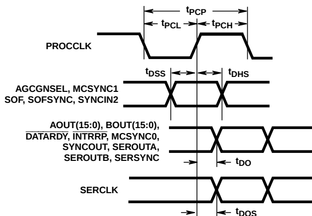
FIGURE 52. TIMING RELATIVE TO PROCCLK
