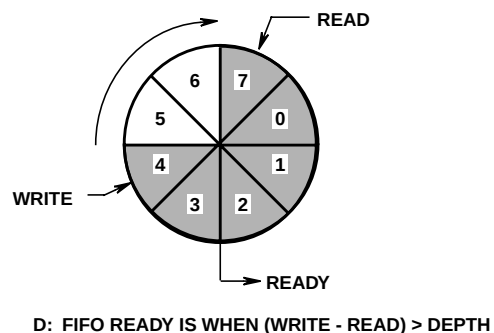
FIGURE 37. FIFO REGISTER OPERATION
