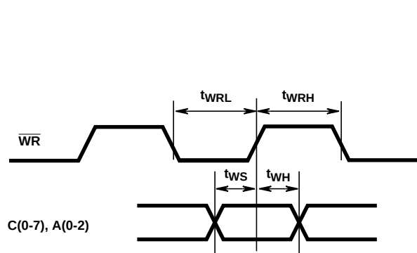
FIGURE 47. TIMING RELATIVE TO \overline{WR}
