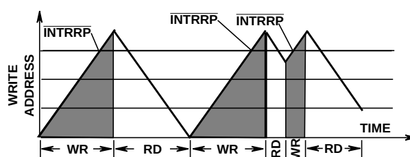
THE THIRD INTERRUPT HAS ONLY 1 NEW DATA ENTRY (INSTEAD OF 3) AT \overline{\text{INTRRP}}
