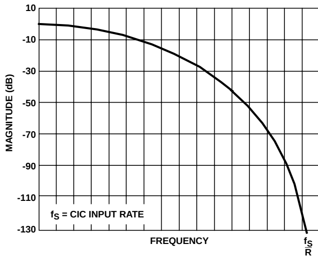
FIGURE 45A. CIC FILTER RESPONSE
