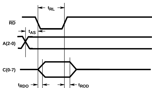
FIGURE 48. TIMING RELATIVE TO \overline{RD}
