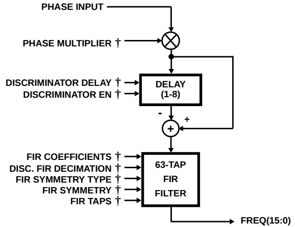
FIGURE 29. FREQUENCY DISCRIMINATOR BLOCK DIAGRAM
