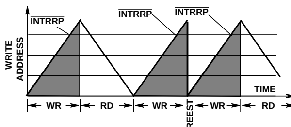
A COMPLETE SET OF 3 DATA SAMPLES IS IN MEMORY AT \overline{\text{INTRRP}}
