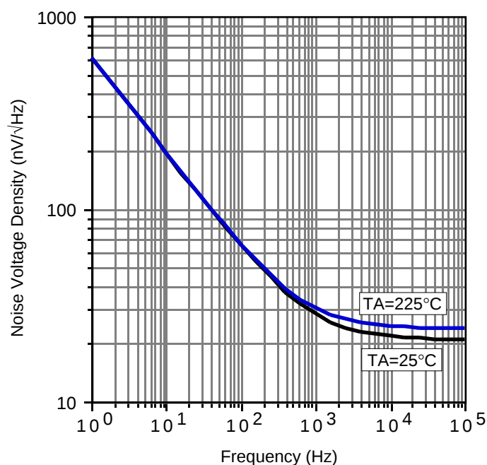
INPUT REFERRED NOISE VOLTAGE vs. FREQUENCY
