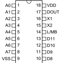
HT12A -18 DIP
