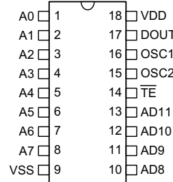
HT12E -18 DIP
