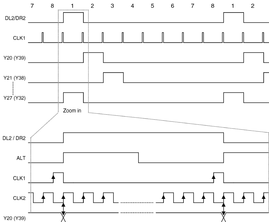
Common data waveform (a typical waveform of channel 2 as a COMMON driver, 1/8 duty)
