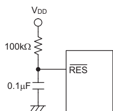
Reset Circuit
