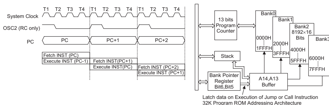
Execution Flow
