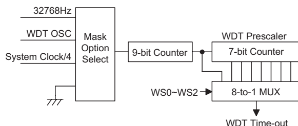
Watchdog Timer
