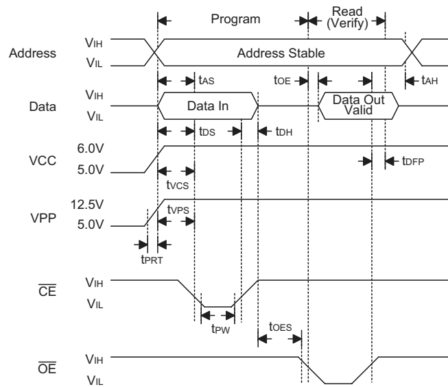
Figure 2. Programming waveforms
