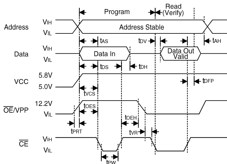
Figure 2. Programming waveforms
