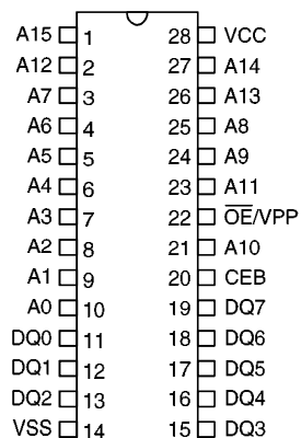
HT27C512 - 28 DIP/SOP
