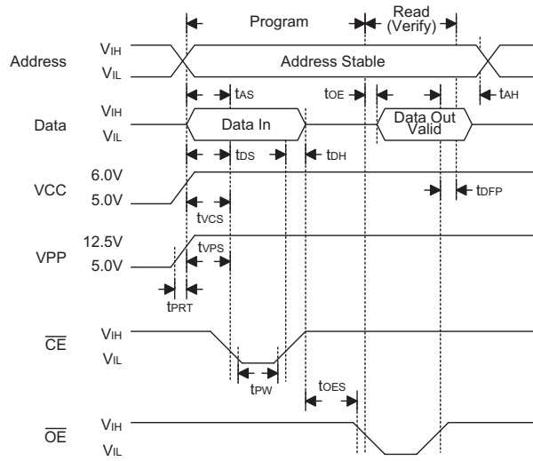
Figure 2. Programming Waveforms
