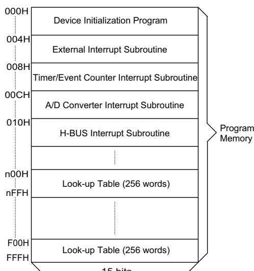
Program memory
