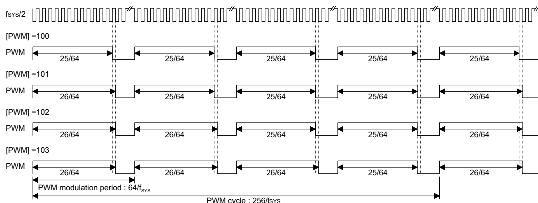
(6+2) PWM mode
