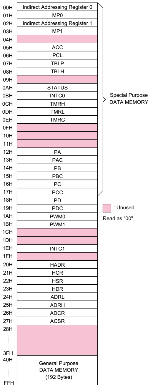
RAM mapping
