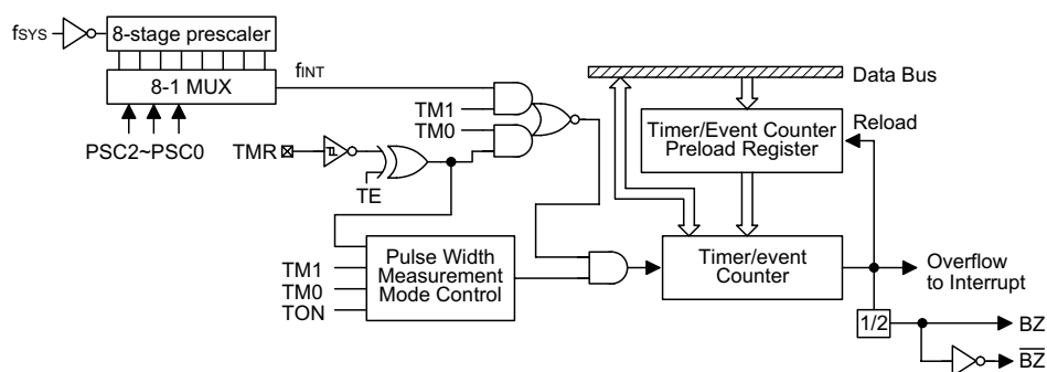
Timer/event counter
