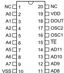
HT6010 -20 DIP/SOP
