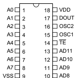
HT6010 -18 DIP
