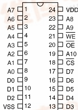
HT6116-70 - 24 DIP/SDIP/SOP
