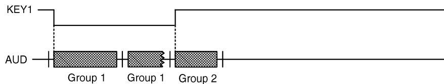
Figure 1 One key two groups function (TWIN mode)
