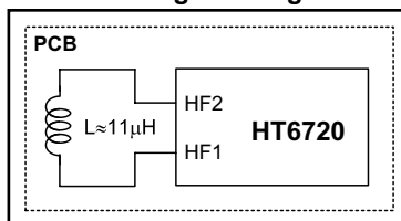
Tag Housing
