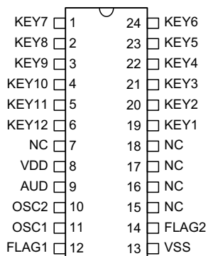
HT817D0 - 24 DIP/SOP
