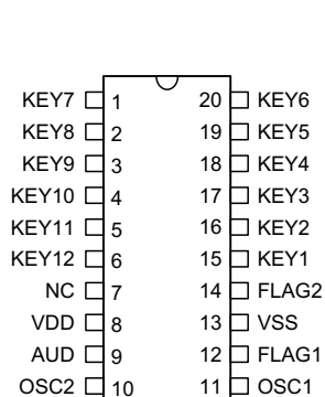
HT817D0 - 20 DIP/SOP
