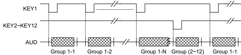
Figure1 Reset of KEY1 playing sequence
