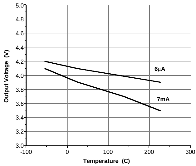
Output drive vs. temperature
