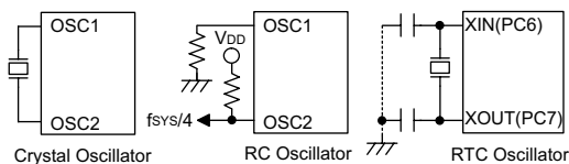
System oscillator
