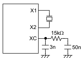
System oscillator circuit
