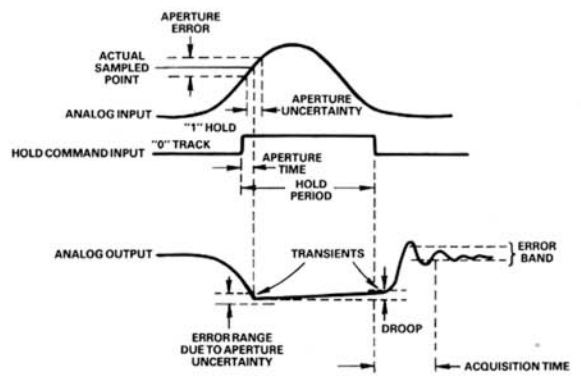
Figure 1. Track/Hold Waveforms – HTC-0300A
