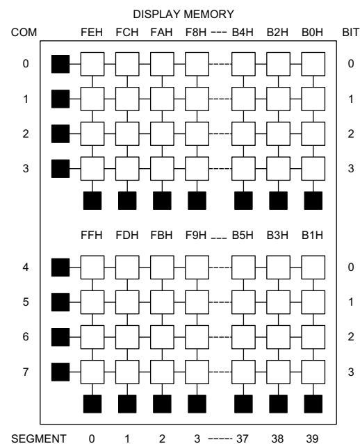
LCD display memory (LCDC0=0)
