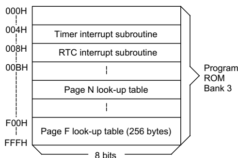
Program memory ROMB=XX11B
