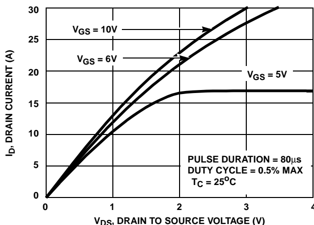
FIGURE 8. SATURATION CHARACTERISTICS
