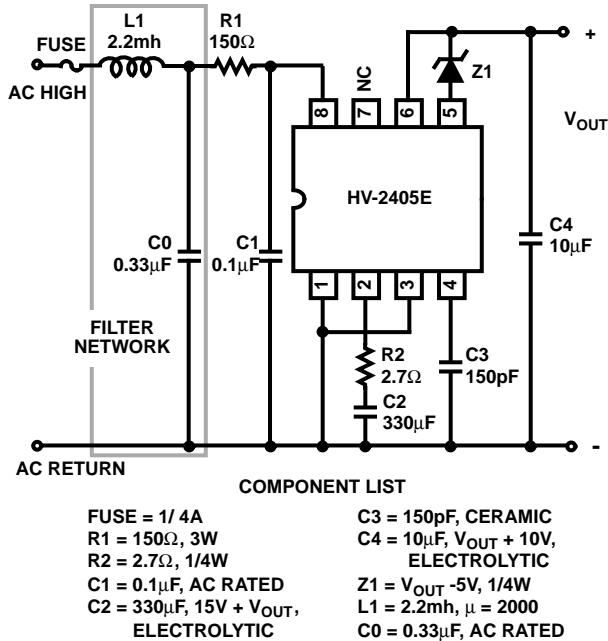
FIGURE 8. IMBEDDED SUPPLY WITH EMI FILTER (I OUT ≤ 30mA)
