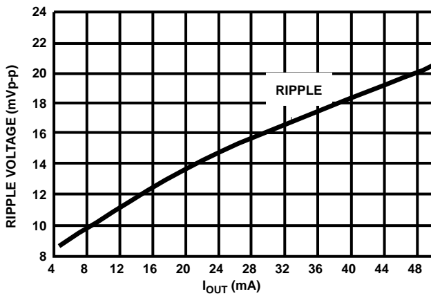
FIGURE 21. OUTPUT RIPPLE VOLTAGE vs LOAD CURRENT
