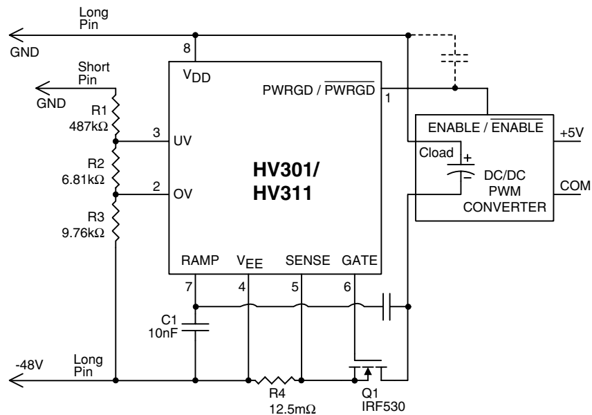
Application Circuit 7
