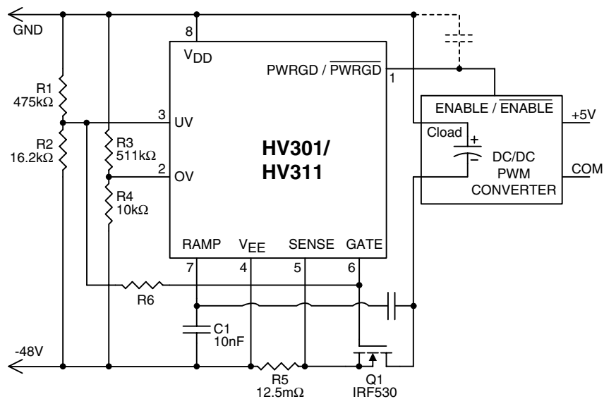
Application Circuit 11
