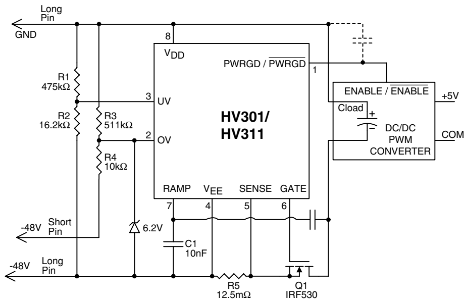
Application Circuit 10
