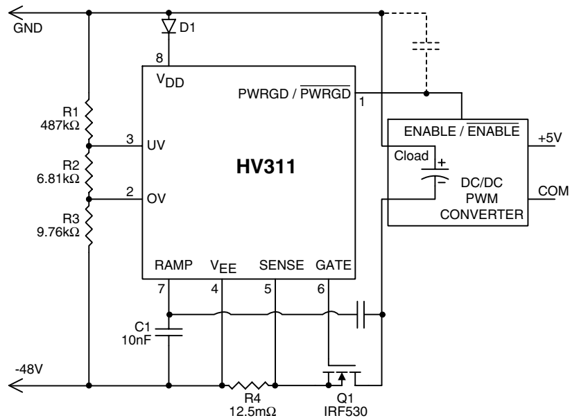
Application Circuit 12
