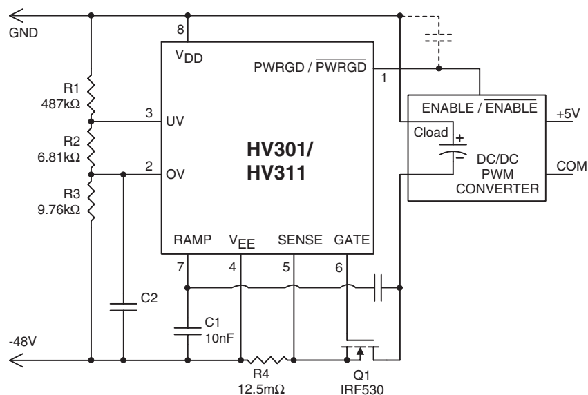
Application Circuit 5
