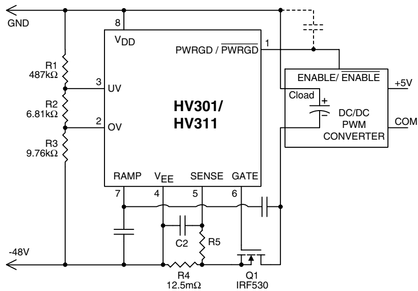
Application Circuit 15
