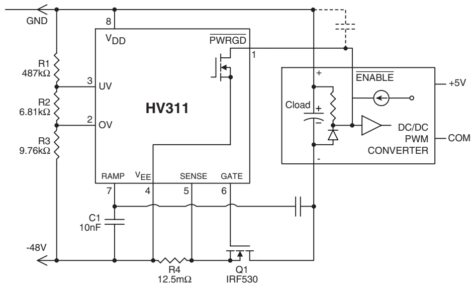
Application Circuit 2
