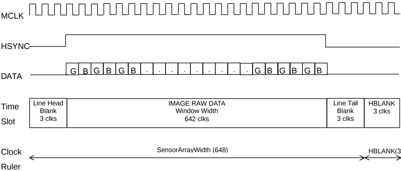
Fig.7 Odd Line Data Timing
